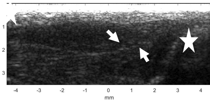
Mouse Sciatic Nerve In-vivo : Three-month old wild type nerve imaged in the left proximal leg. Top: Raw image, arrowheads point towards fascicles, star = femur Bottom: whole nerve outline in red, fascicles outlined in yellow. Imaged using Verasonics 64LE beamformer, with Verasonics 35-16vX transducer. Castoro Lab 2022
